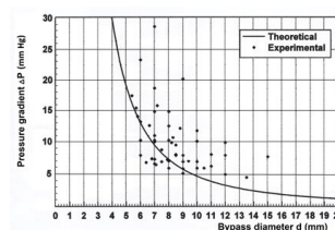
Figure 1) The curve showing the relationship between the required minimal pressure gradient and crossover bypass graft diameter.
