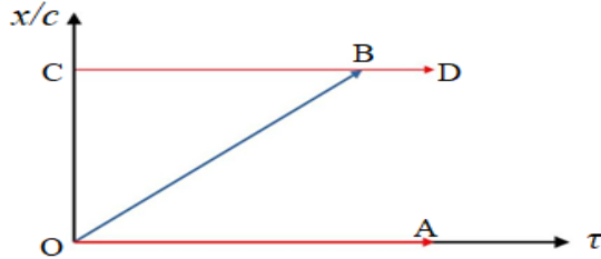
Figure 1) Following the three relevant clocks of the TT case; (travel to the star). The perspective of the earth
