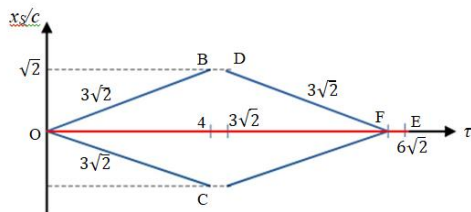
Figure 3) Event graphs for the two rockets; in the perspective of the symmetric RF, K_S
