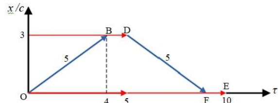
Figure 2) Event graphs of the twins in the perspective of the earth-based RF, K. The blue graphs describe the travelling twin's journey. The red line, OE follows the earthbound twin, having x/c \equiv 0
