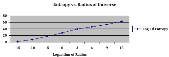
Figure 1) Entropy vs. Radius of the Universe
