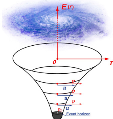
Figure 6: The so-called supermassive black hole is only a deep potential well formed by galaxies at its center.
