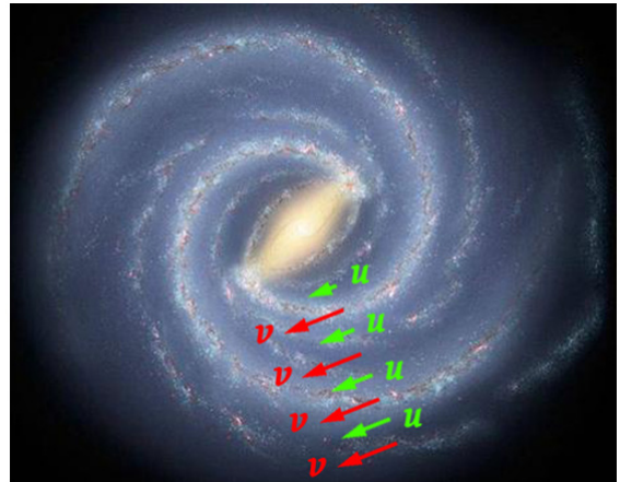
Figure 4: The etheric absolute frame of reference formed within the rotating galaxy: u is the rotation speed of the absolute reference frame of the galactic ether; v is the rotation speed of the stars in the galaxy.
