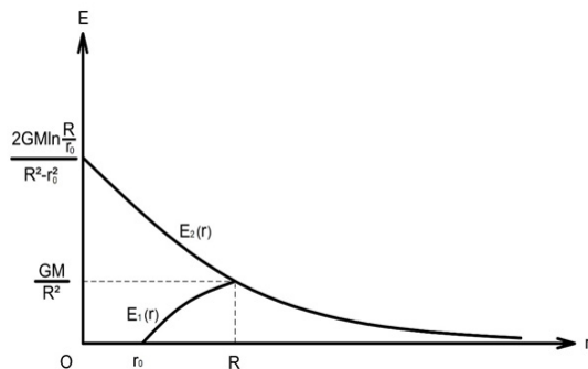
Figure 3: The functional relationship between E_1(r) and r .
