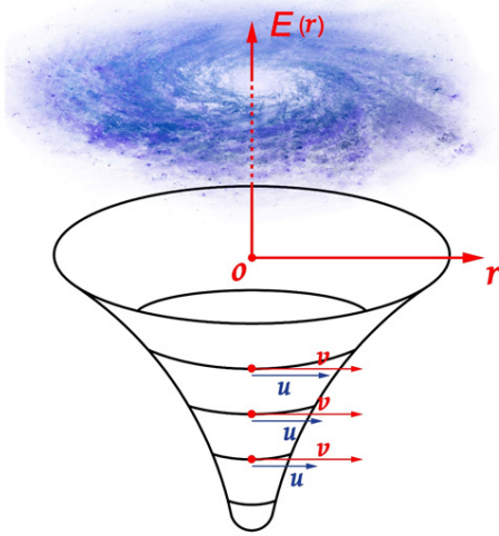
Figure 5: The etheric absolute frame of reference formed within the rotating galaxy: u is the rotation speed of the absolute reference frame of the galactic ether; v is the rotation speed of the stars in the galaxy.
