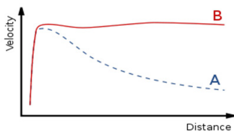
Figure 1. The relationship between the speed of a star's rotation around the galaxy and its distance from the galaxy's center.
