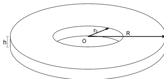
Figure 2: Simplified geometry of galaxies: A thin disk with mass M , mass density \rho , outer radius R , inner radius r_0 , and thickness h .
