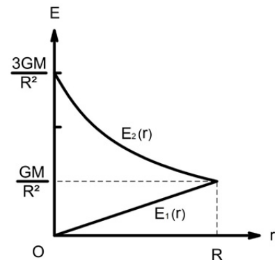
Figure 7: The functional relations of E_1(r) , E_2(r) and r .
